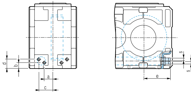
Water connection for cooling coil without cooling water controller
